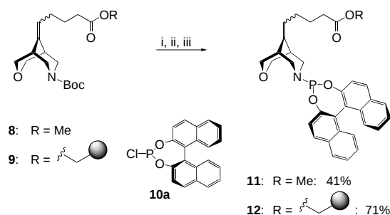
Scheme 3. Synthesis of phosphoramidites 11 and 12 : i) TFA, CH 2 Cl 2 , 0.5 h, RT, quant.; ii) Et 3 N CH 2 Cl 2 (only for 9 ); iii) 10a , Et 3 N, toluene, 12 h, RT.
