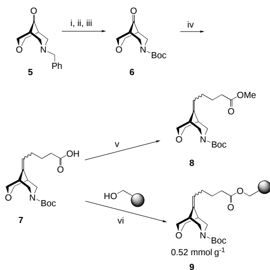
Scheme 2. Synthesis of the model systems 8 and 9 : i) \text{ClCOOCH}(\text{Cl})\text{CH}_3 , \text{CH}_2\text{Cl}_2 , \Delta , 2 h; ii) \text{MeOH} , \Delta , 2 h; iii) \text{Boc}_2\text{O} , \text{KOH} , \text{H}_2\text{O} , dioxane, RT, 12 h, 87 %; iv) \text{BrPh}_3\text{P}(\text{CH}_2)_4\text{COOH} , \text{KOtBu} , THF, 0^\circ\text{C} \rightarrow \text{RT} , 2.5 h, 54 %; v) EEDQ, \text{MeOH} , RT, 12 h, 82 %; vi) DIC, DMAP, \text{CH}_2\text{Cl}_2 , 12 h, RT, 71 %, then \text{Ac}_2\text{O} , pyridine.
