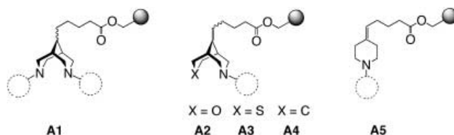
Figure 1. (Hetero-)bispidines A1–A4 and piperidine A5 as ligand backbones.
