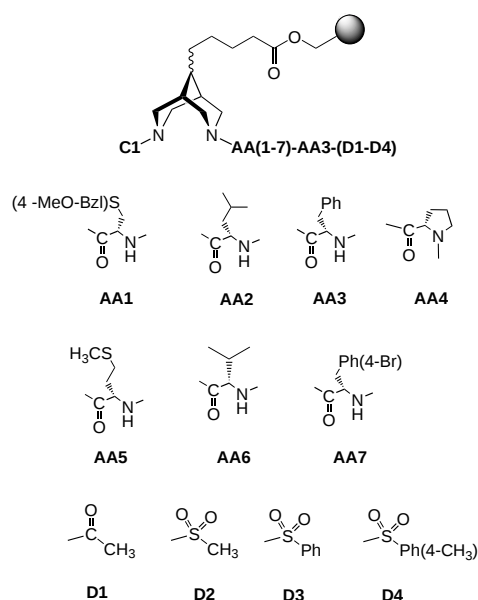
Figure 4. Amino acid and dipeptide substituted ligands.
