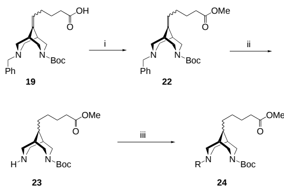
Scheme 8. Model reactions with bispidine system 23 : i) EEDQ, MeOH, 12 h, RT, 75%; ii) \text{H}_2 , Pd/C, EtOH, 12 h, RT, 90%; iii) various reactions and conditions.
