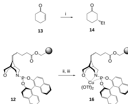
Scheme 6. Modified reaction conditions for the conjugate addition with ligand 12/16 : i) Et 2 Zn, 16 toluene, CH 2 Cl 2 , 0 °C, complete conversion 37–40 % ee; ii) 5 equiv Cu(OTf) 2 , CH 2 Cl 2 /3 % DMF; iii) washing.
