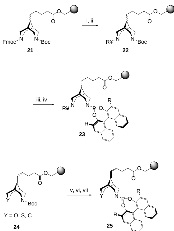
Scheme 9. Synthesis of solid phase ligands 23 and 25 : i) Piperidine; ii) modification at the N atom; iii) TFA, \text{CH}_2\text{Cl}_2 , \text{NEt}_3 ; iv) CIP( \text{R}_2 BINOL) \text{Et}_3\text{N} , toluene; v) TFA, \text{CH}_2\text{Cl}_2 ; vi) \text{CH}_2\text{Cl}_2 , \text{NEt}_3 ; vii) CIP( \text{R}_2 BINOL) \text{Et}_3\text{N} , toluene.
