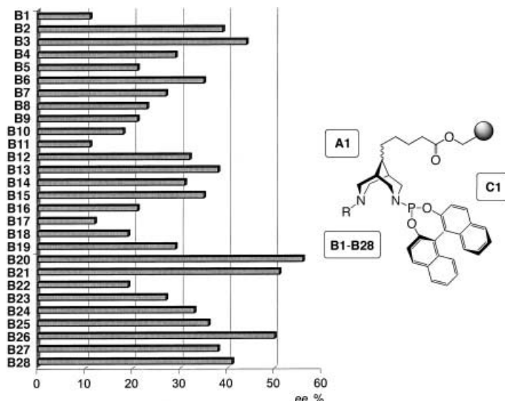
Figure 5. ee Values determined with ligand combinations A1–B(1–28)–C1 .
