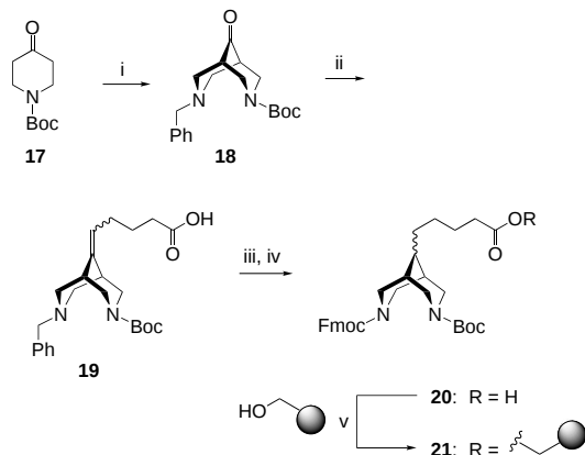
Scheme 7. Synthesis of bispidine 20 and coupling to the solid phase: i) \text{PhCH}_2\text{NH}_2 , (\text{HCHO})_n , AcOH, MeOH, 65^\circ\text{C} , 4 h, 81%; ii) \text{BrPh}_3\text{P}(\text{CH}_2)_4\text{COOH} , \text{KOtBu} , THF, 0^\circ\text{C} \rightarrow \text{RT} , 2.5 h, 68%; iii) \text{H}_2 , Pd/C, EtOH, 12 h, RT, quant.; iv) FmocCl, \text{NaHCO}_3 , THF, \text{H}_2\text{O} , 12 h, RT, 69%; v) DIC, DMAP, \text{CH}_2\text{Cl}_2 , 12 h, RT, 94% ( 0.61 \text{ mmol g}^{-1} ).
