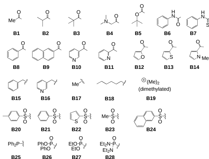
Figure 2. Building blocks for the ligand library: nitrogen substituents B1–B28 .
