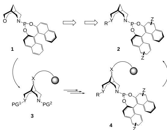
Scheme 1. Solid-phase optimisation strategy for bispidine phosphoramidites 1 and 2 .
