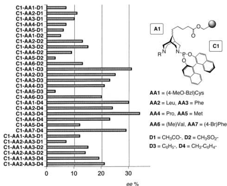
Figure 6. ee Values determined with amino acid ligands incorporating substituted amino acids or dipeptides.
